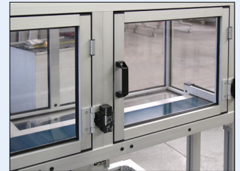
Aluminum Framing
